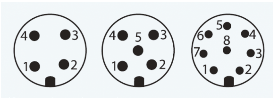
M12 Contact Inserts, male connector, view onto connection side
